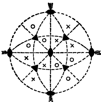
Symmetry of Tetartohedral Class
